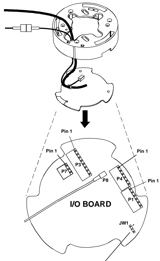
Figure 15. Electrical connections
