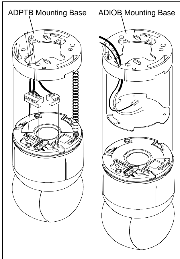
Figure 2. Mounting base and housing and eyeball assembly
