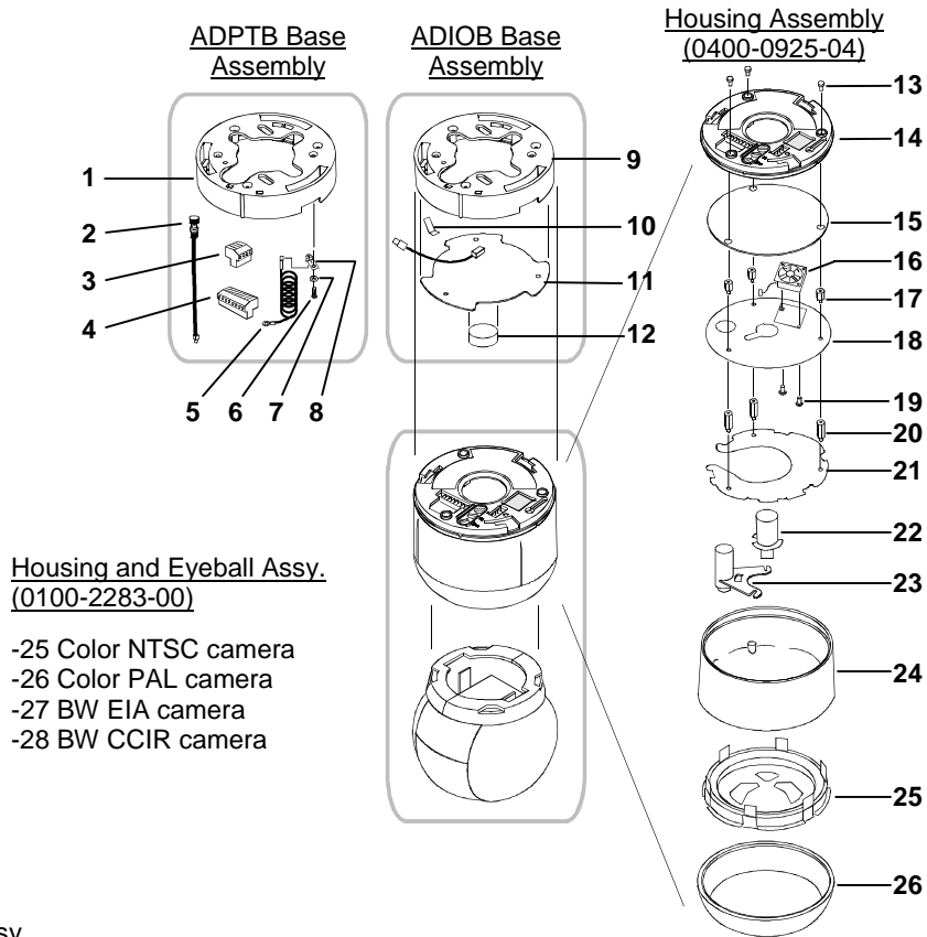
Figure 37. Base, housing, and eyeball assembly
