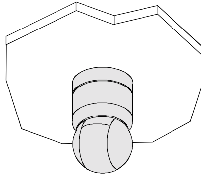
Figure 4. Surface mounting to tile ceilings
