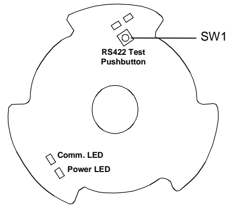
Figure 16. Test switch/LEDs on I/O board
