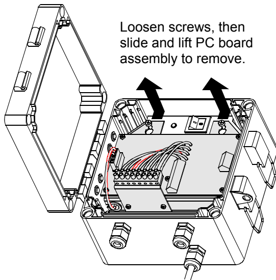
Figure 5. Accessing connections
