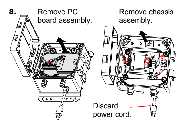
Figure 4. Pole-mount—details
