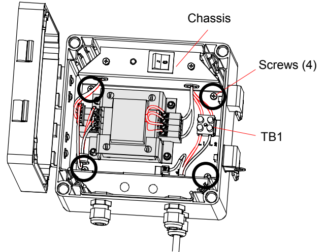
Figure 6. Transformer compartment detail
