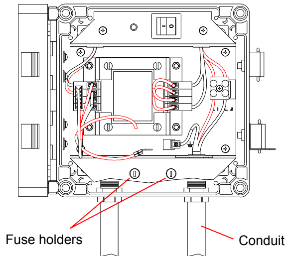
Figure 7. Conduit attachment
