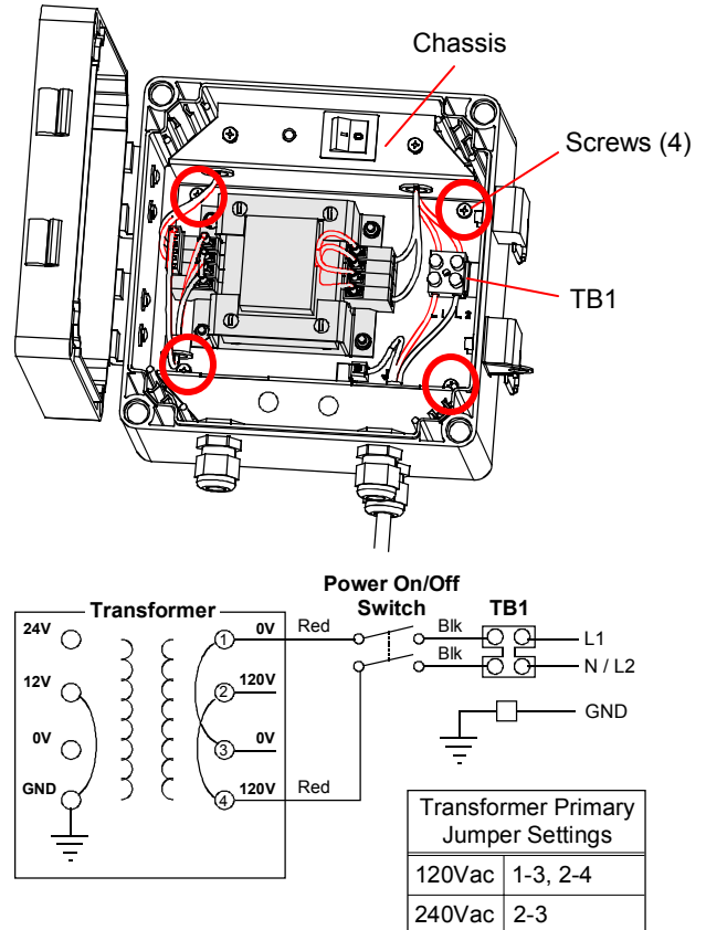
Figure 6. Transformer compartment detail
