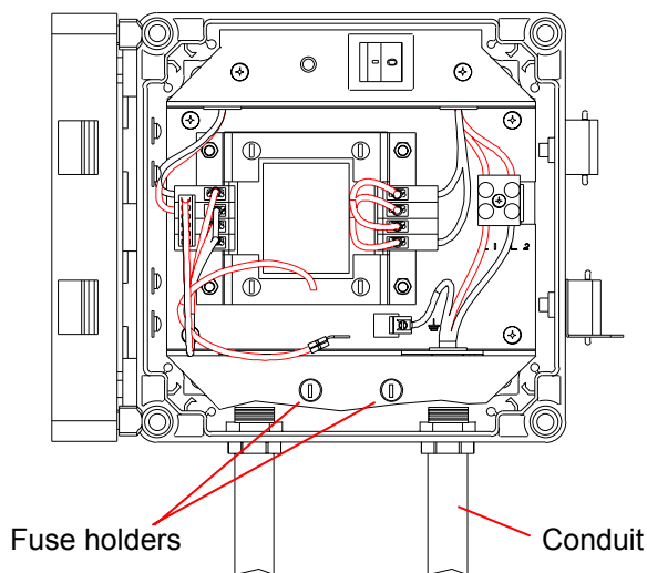
Figure 7. Conduit attachment
