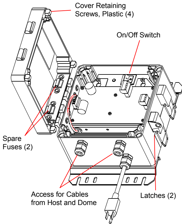
Figure 1. SensorNet J-Box
