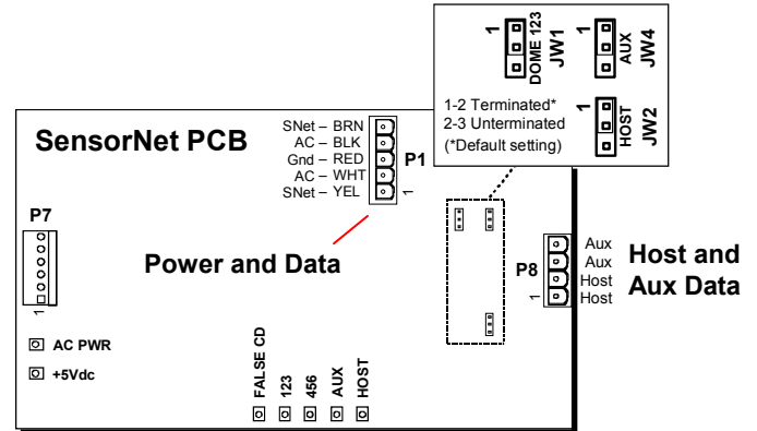
Figure 8. PCB connectors and jumpers
