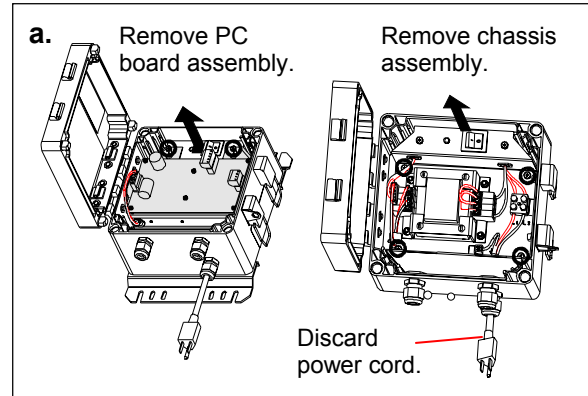
Figure 4. Pole-mount—details
