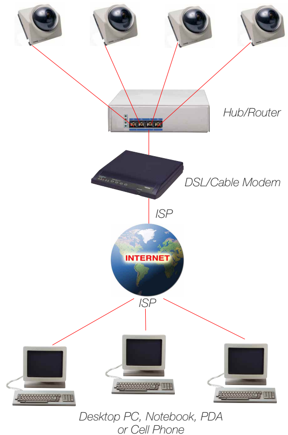
Connection Example 2*
