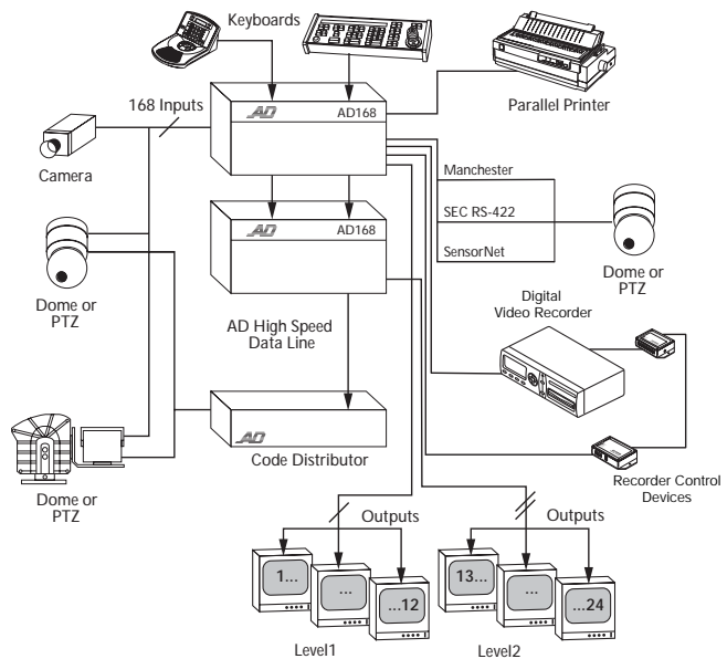
MegaPower 168 Series Typical System Connections
